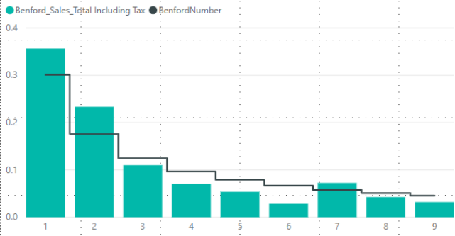
Benford_Sales_Total Including Tax and BenfordNumber by Number and Package
