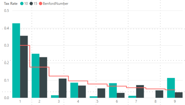
Benford_Sales_Total Including Tax and BenfordNumber by Number and Tax Rate
