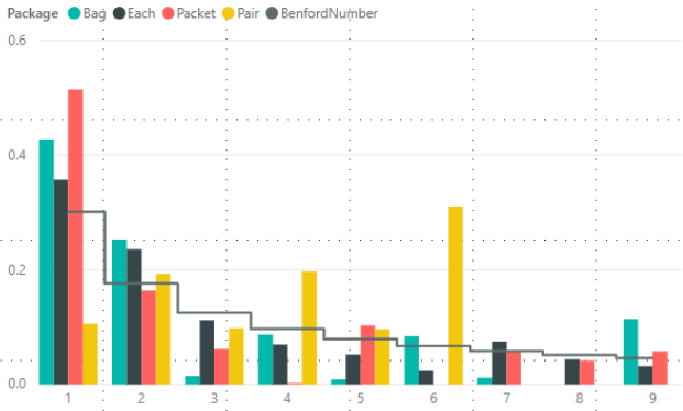
Benford_Sales_Total Including Tax and BenfordNumber by Number and Package
