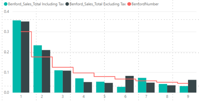
Benford_Sales_Total Including Tax, Benford_Sales_Total Excluding Tax and BenfordNumber by Number
